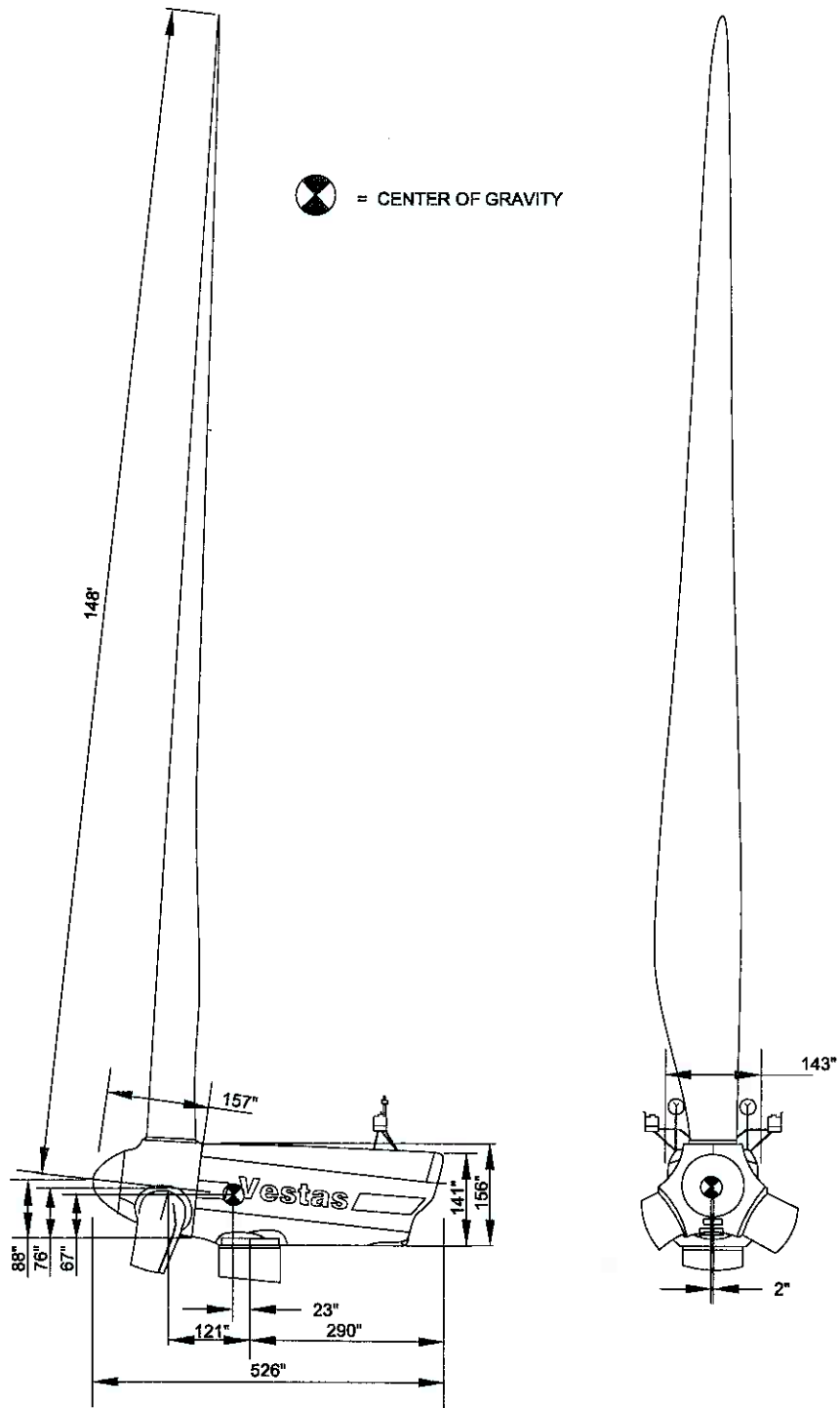
FIGURE SOURCE: VESTAS V-90 CATALOG CUT
